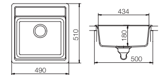
Ref. NEMO N-100 S Nemo single bowl
