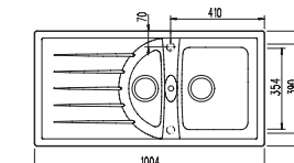
Ref. GEN D 150 Genius 1.5 bowl and drainer
