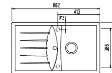
Ref. GEN D 100 Genius single bowl and drainer
